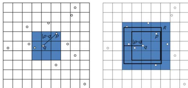
Fig. 1 Grid method in YPK-CkNN
