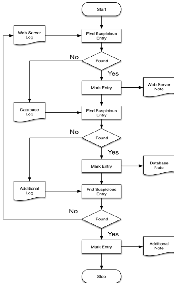
Fig. 2 Log analysis flowchart
