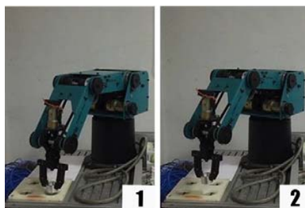
Fig. 10 Arm picking up the object
