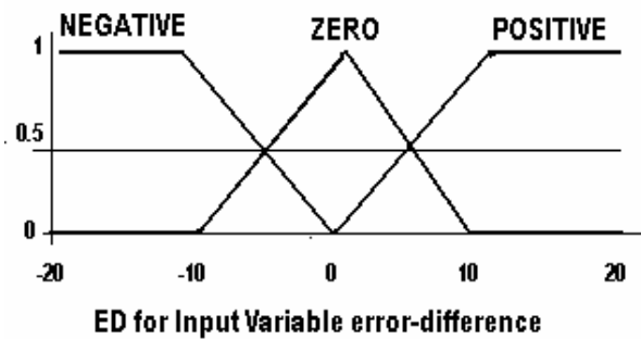
Fig. 1 Membership Function
