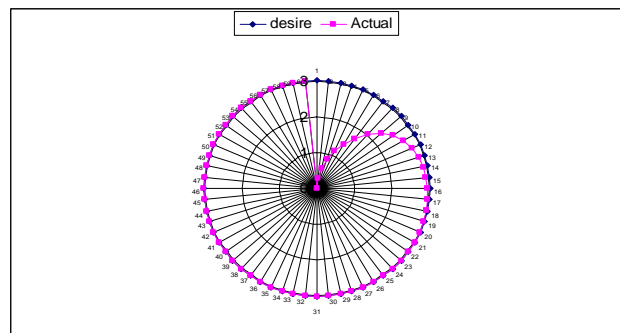
Fig. 4 Step Response of Proportional Controller
