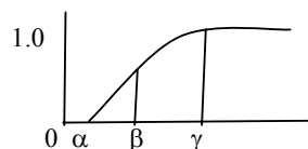
Fig. 4 One typical form of the S-shaped membership function
