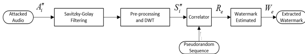
Fig. 2 Structure of extraction scheme
