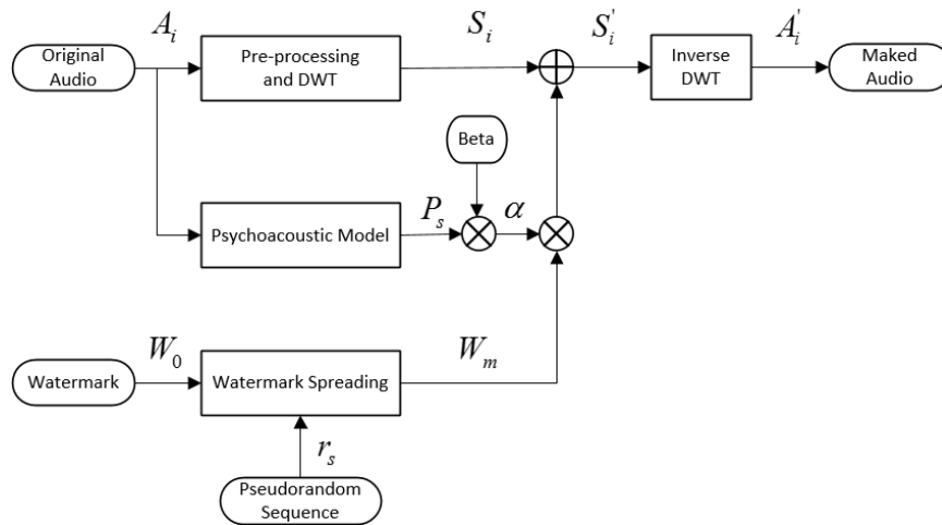
Fig. 1 Structure of Embedding Scheme
