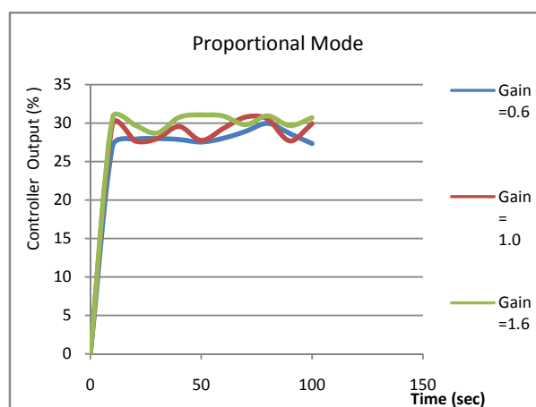
Fig. 2 Effect of gain on controller output for P-mode
