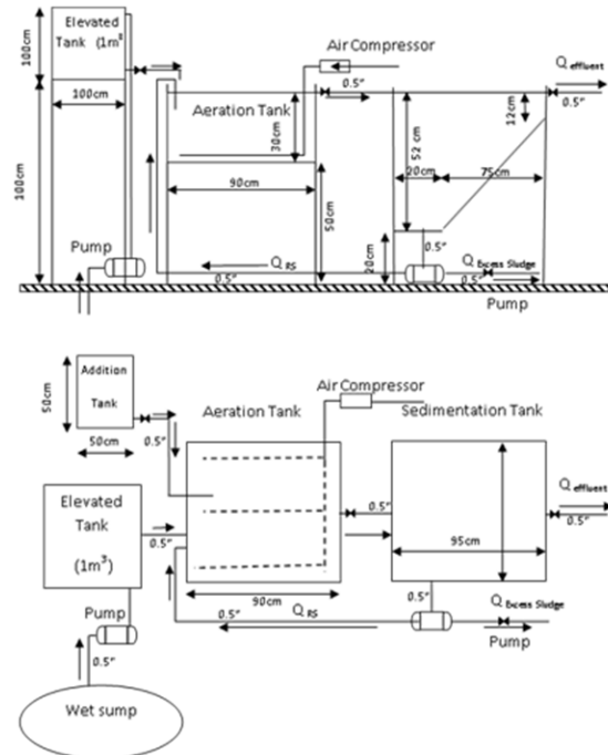
Fig. 1 A-stage process
