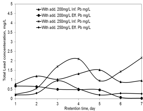
Fig. 9 Influent and Effluent Pb during the second group (with 200 and 250mg/L Alum. salts addition)
