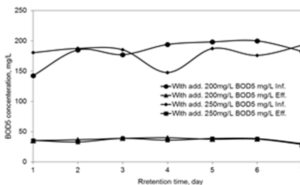
Fig. 4 Influent and Effluent BOD 5 during the second group (with 200 and 250mg/L Alum. salts addition)
