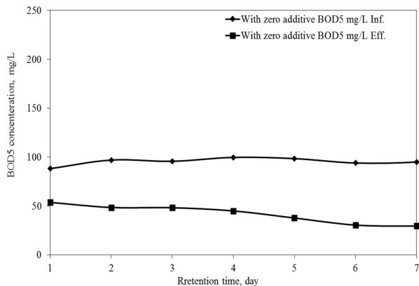
Fig. 2 Influent and Effluent BOD 5 during the first group (zero additives)
