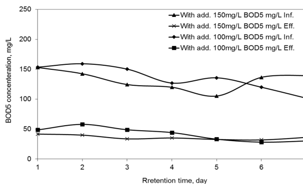
Fig. 3 Influent and Effluent BOD 5 during the second group (with 100 and 150mg/L Alum. salts addition)
