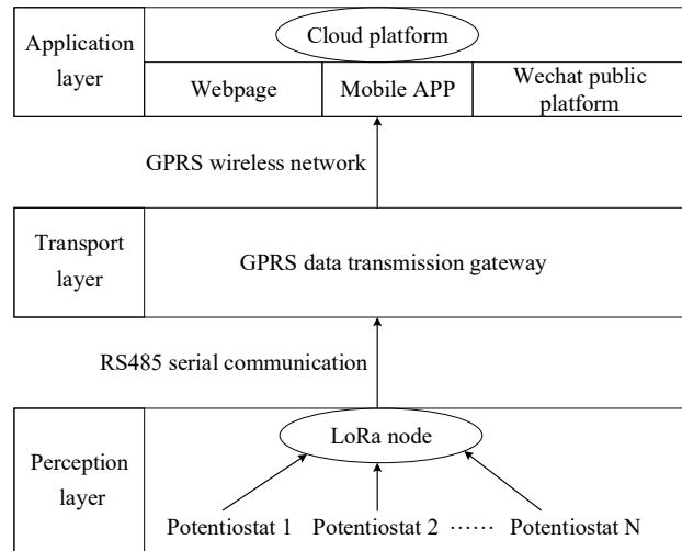
Fig. 2 System overall structure design block diagram
