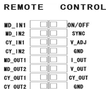
Fig. 1 Remote interface diagram of a KTCP-3 potentiostat
