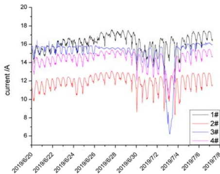
Fig. 8 Current real-time curve
