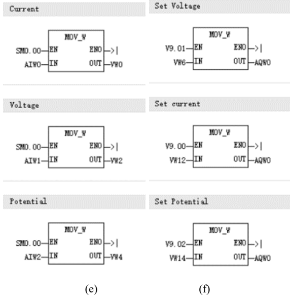
Fig. 3 PLC program for remote monitoring of potentiostat
