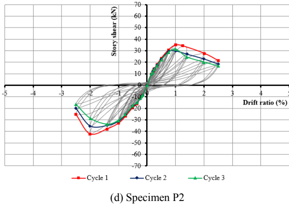
Fig. 8 Column shear force – drift ratio relation
