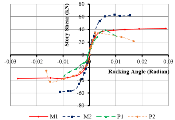
Fig. 12 Rocking Angle
