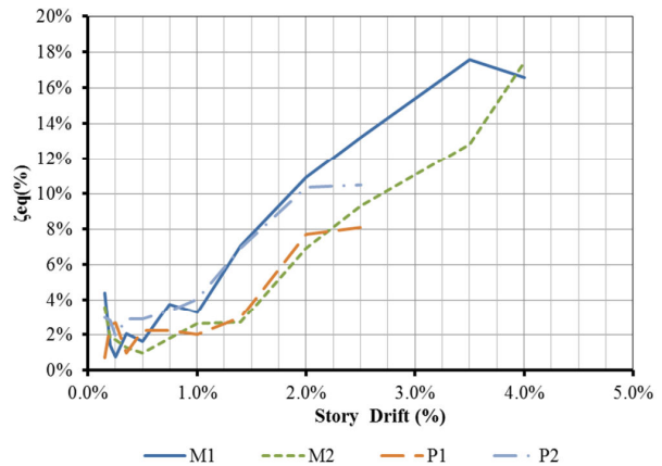
Fig. 13 Energy dissipation
