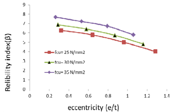
Fig. 8 Relation between reliability index ( \beta ) and eccentricity ( e/t ) for 500*500 mm 2 Concrete cross section, \mu=2.80\% and f_y=420 MPa
