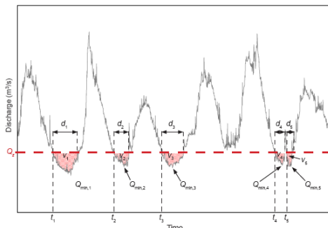
Fig. 2 Illustration of common hydrological drought characteristics (after Fleig et al. 2006)
