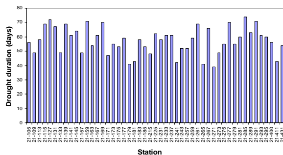
Fig. 4 2-year drought duration of all stations
