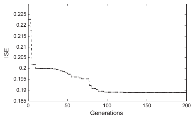
Fig. 6. Convergence of objective function for example-2
