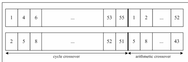
Fig. 3 Crossover operator for Hsiao code
