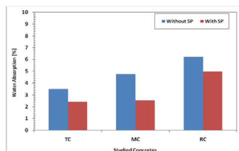
Fig. 10 Water absorption of studied concretes
