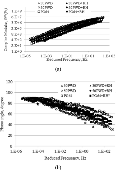
Fig. 3 (a) Master curve of complex modulus, (b) Master curve of phase angle
