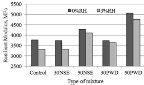
Fig. 5 Effect of RH-WMA on the resilient modulus
