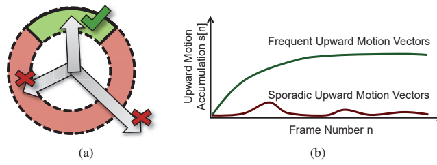
Fig. 2 (a) Motion vectors in the upper quarter with an appropriate length are allowed, others are rejected (b) Accumulation difference for frequent and sporadic upward motions
