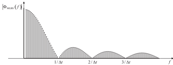
Fig. 3. Shape of power spectrum of MLBS.
