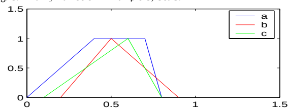
Fig. 6. Fuzzy numbers in Example 3, Set 4.
