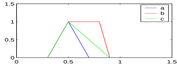
Fig. 5. Fuzzy numbers in Example 3, Set 3.
