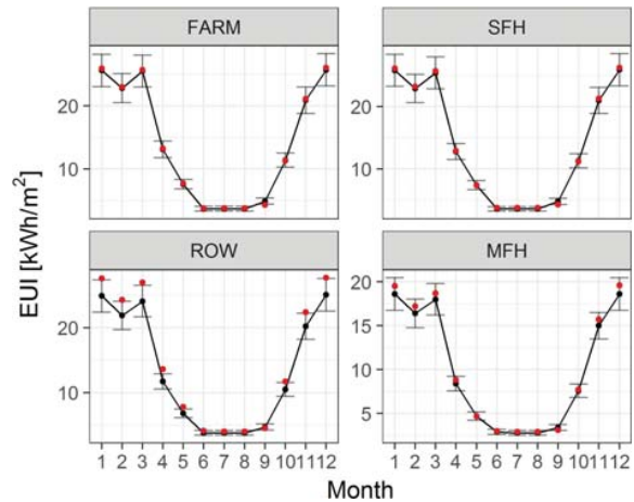
Fig. 5 Monthly heat demand (EUI) in buildings built between 1961 and 1972 (construction period P5). The error bars denote the mean value of the individual buildings \pm 10\% . The red dots denote the heat demands calculated in the comprehensive archetype model
