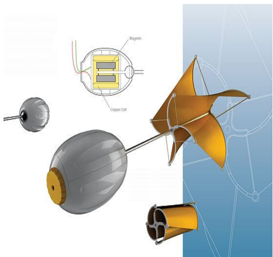
Fig. 3 Design of hydraulic propulsor and electric generator and micro HPP “VENA”
