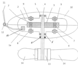
Fig. 10 Design of mobile micro HPP (section view along the rotation axis)
