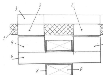
Fig. 6 Mutual arrangement of RMS and SEMS in electric generator
