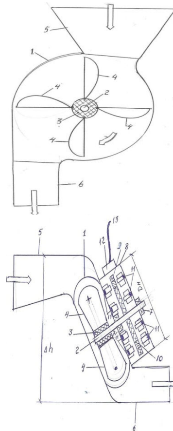
Fig. 9 Option for design of the micro HPP [13] without electric generator (at the left) and section view along the hydraulic drive rotation axis (on the right)
