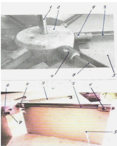
Fig. 11 Design of hydraulic drive with rotary blades
