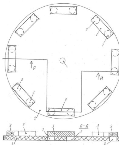
Fig. 5 Electric Generator Disc Rotor Structure [8]
