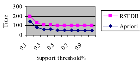
Fig. 3 Time Complexity Graph for TDB1
