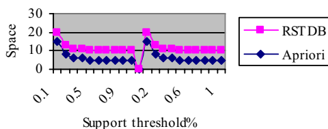
Fig. 2 Space complexity Graph for TDB1
