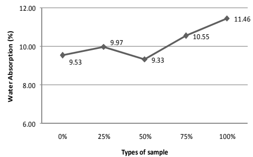
Fig. 4 The average water absorption of cement and sand bricks with recycled fine aggregate
