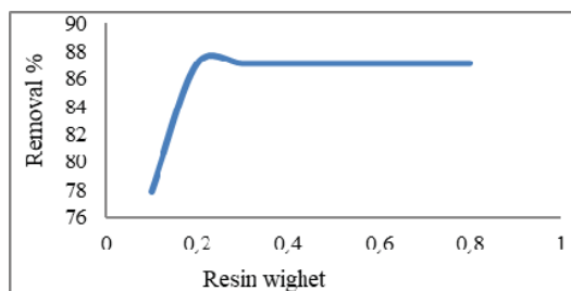
Fig. 11 The effect of resin dosage on the exchange of calcium ion by sulfonated waste polystyrene resin
