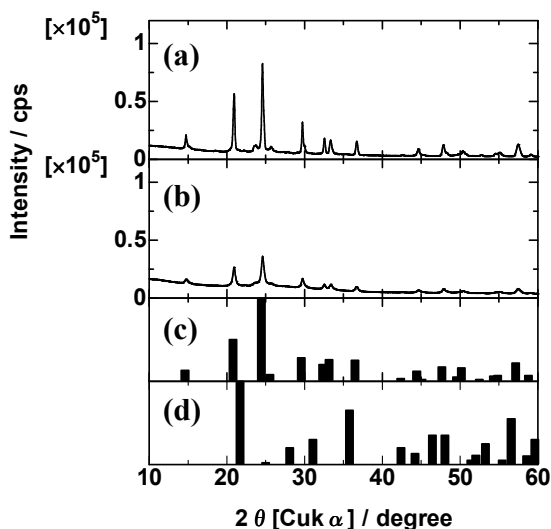
Fig. 1 XRD patterns of precursor powder heated at 800°C for 30 min before and after the ball-milling (a) Before the ball-milling, (b) After the ball-milling, (c) Standard pattern of \text{LiTi}_2(\text{PO}_4)_3 , (d) Standard pattern of \text{AlPO}_4
