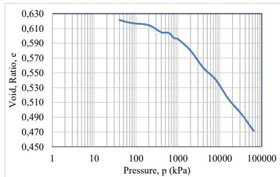
Fig. 8 Compression curve for USB3 sample
