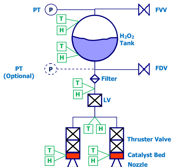
Fig. 1 The RCS-DM configuration for the NB satellite
