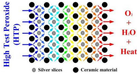
Fig. 2 Design concept of composite silver catalyst bed
