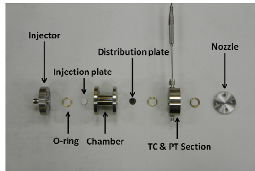
Fig. 3 Main parts of the H_2O_2 thruster
