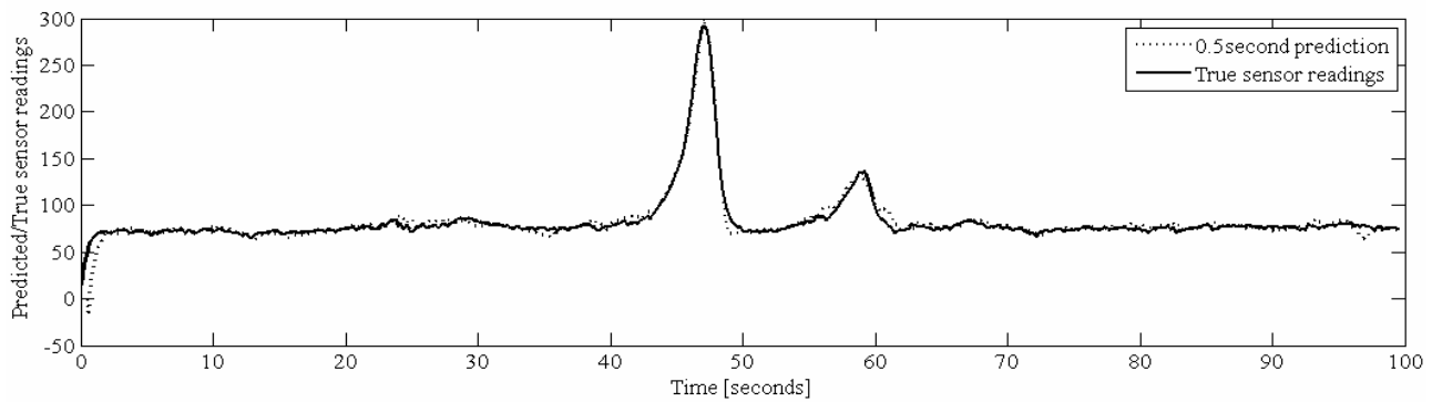
Fig. 7 Predicted vs true sensor readings for one sensor during the validation experiment, prediction horizon = 0.5 second
