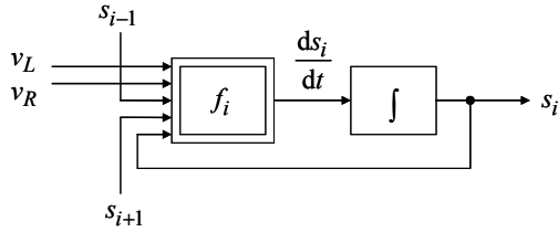
Fig. 4 Block diagram of the model for one sensor
