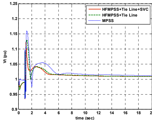
Fig. 14 Terminal voltage of machine 1
