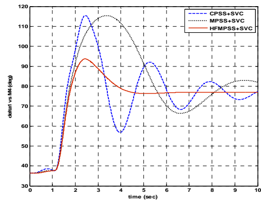
Fig. 15 Rotor angle deviation of machine 1 w.r.t. machine 4
