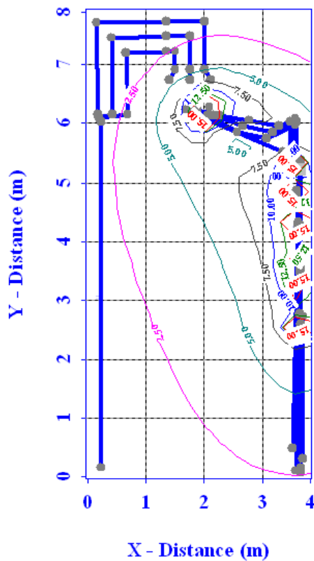
Fig. 8. Contour presentation of simulated magnetic field
