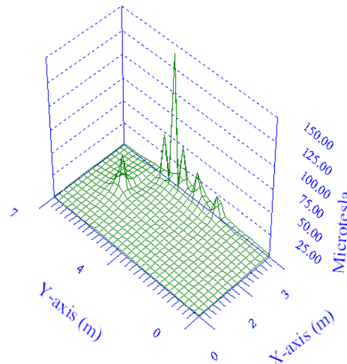
Fig.7. 3D presentation of simulated magnetic field
