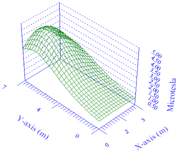
Fig. 11 3D presentation of simulated magnetic field at height 1m above the first floor
