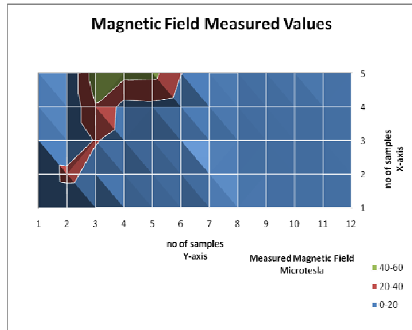
Fig. 6 Contour Plot for the Measured Magnetic Field
