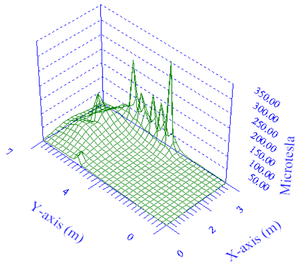
Fig. 10. 3D presentation of simulated magnetic field at peak load
