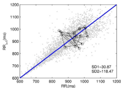
Fig. 3 Poincaré plots with similar SD1 and SD2 having different temporal dynamics. Two different RR interval time series of length N ( N = 2000 ) with similar SD1 and SD2 values having different temporal dynamics (first 20 points) are shown in top and bottom panel
