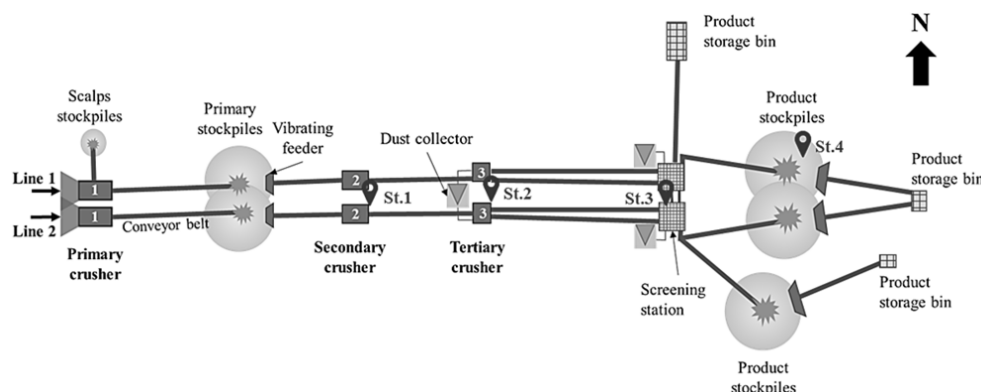
Fig. 2 The schematic crushing process at mine A
