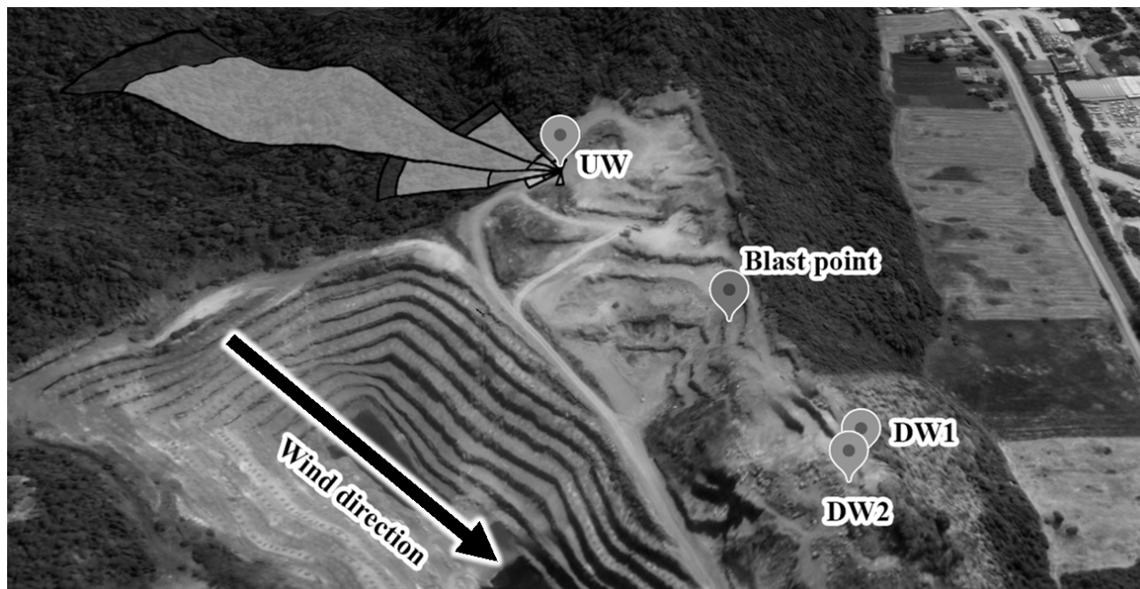
Fig. 4 Sampling points of the blasting zone
