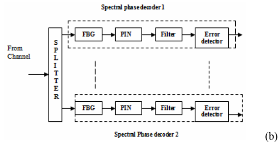
Fig. 1 Simulation setup of the proposed scheme (a) Transmitter (b) Receiver
