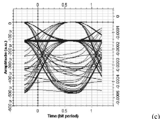
Fig. 2 Eye diagram of (a) one of the RD channels, (b) one of the Hadamard channels, and (c) one of the MFH channels, at 10 G bit/s
