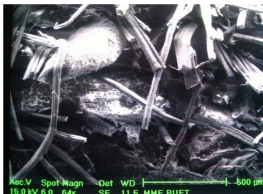
Fig. 13 Tensile fracture surface of 20% jute-coir fiber reinforced hybrid polypropylene composite
