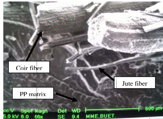
Fig. 10 Tensile fracture surface of 5% jute-coir fiber reinforced hybrid polypropylene composite
