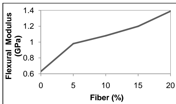
Fig. 7 Variation of flexural modulus at different fiber content.
