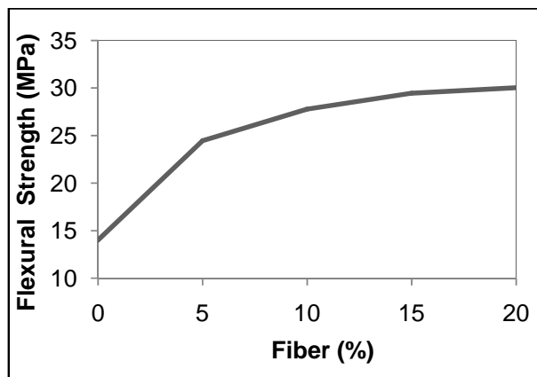
Fig. 6 Variation of flexural strength at different fiber content.
