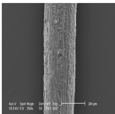
Fig. 3 SEM image of coir fiber [11]
