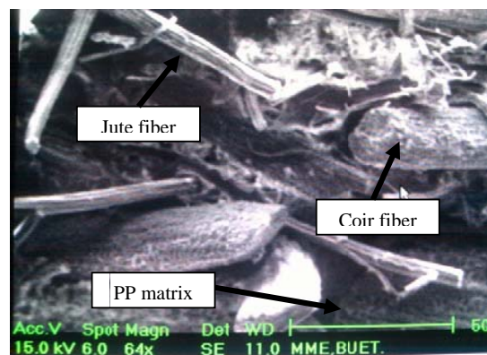
Fig. 12 Tensile fracture surface of 15% jute-coir fiber reinforced hybrid polypropylene composite
