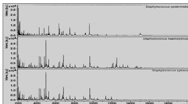
Fig. 4 MALDI-TOF-MS profiles of three isolates of Coagulase negative staphylococci ( S. epidermidis , S. haemolyticus and S. xylosum ) cultured overnight at 37°C on Columbia blood agar plates
