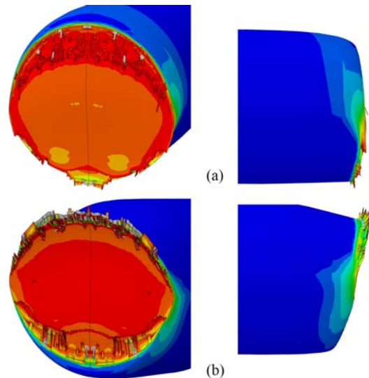
Fig. 7. The damage parameter fields of Extended Mohr–Coulomb criterion [2] after the cutting process simulation for: (a) rod stock; (b) shred
