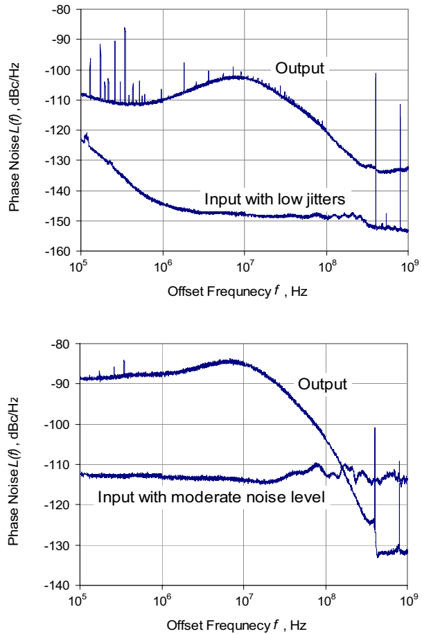
Fig. 4 Variations in output phase noise with low and moderate levels of input jitters.
