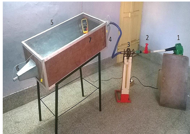
Fig. 2 Experimental setup of solar air collector system
