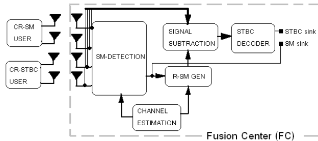
Fig. 4 Hybrid-MIMO receiver scheme (HMRS)
