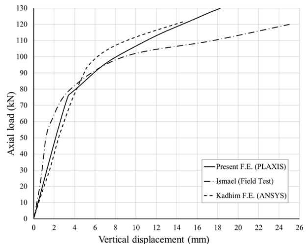
Fig. 2 Comparison between present finite element results and the results of [23] and [17]
