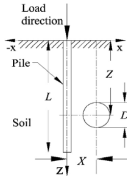
Fig. 3 Geometry of pile on cavited soil with details of parameters.
