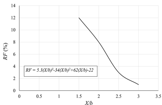
Fig. 8 Variation of RF % various X/b , ( D/b=2 , Z/L=0.8 ).
