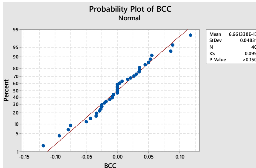
Fig. 1 Results of normality test for BCC model
