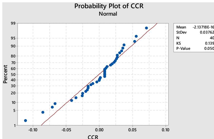
Fig. 2 Results of normality test for CCR model
