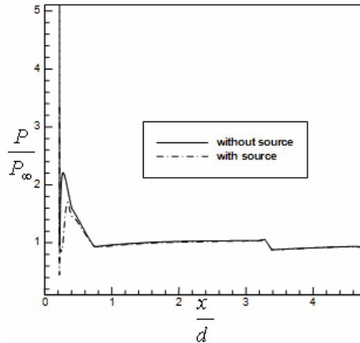
Fig. 16 Pressure distribution over the cowl
