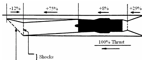
Fig. 1 Example of thrust distribution over a supersonic engine installation at M_\infty=2.2 , [1]
