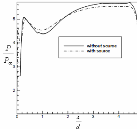
Fig. 17 Pressure distribution over the spike
