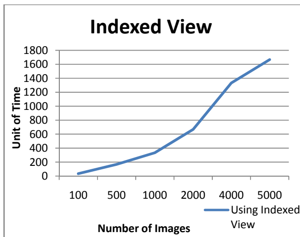
Fig. 8 Time Complexity Analysis Using Indexed View
