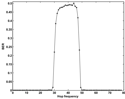
Fig. 3 Performance of HV1 packets
