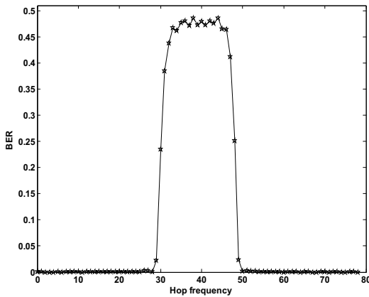
Fig.4 Performance of HV2 packets
