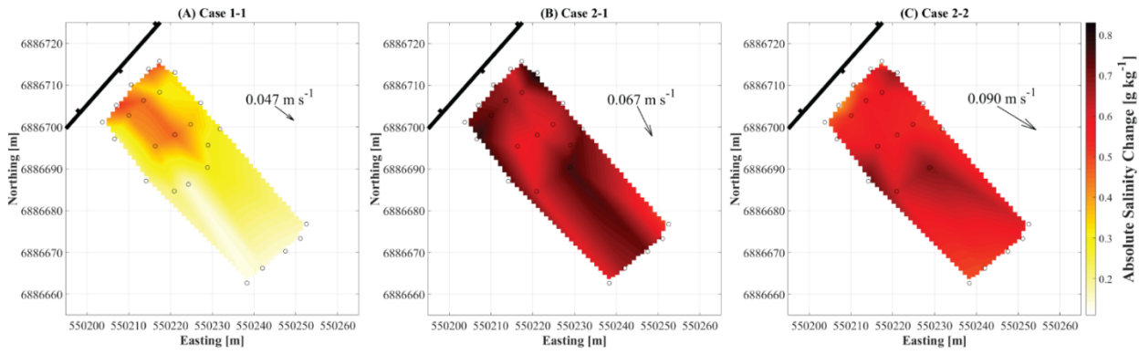
Fig. 4 Mean change in absolute salinity over experiment durations at 2.5 m elevation above seafloor. Mean current velocity vector coinciding with 2.5 m elevation also presented. Spatial linear interpolation is used between measured sensor locations (open black circle symbols)
