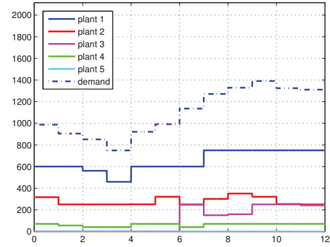
Fig. 3 Example of power allocation among the plants
