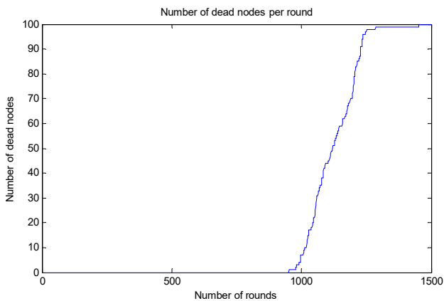
Fig. 5 Number of dead node for Eo = 0.5
