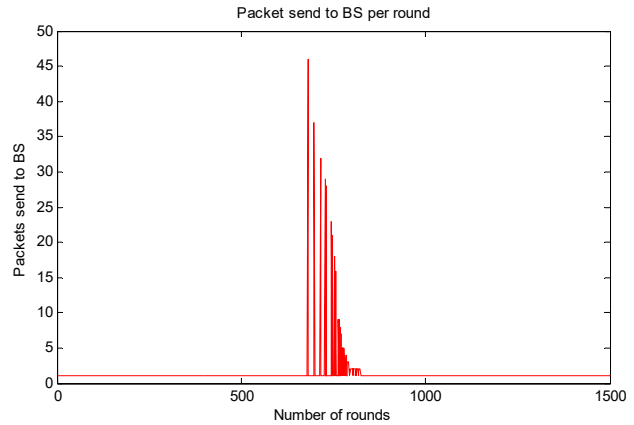
Fig. 6 Throughput of the network for Eo = 0.3
