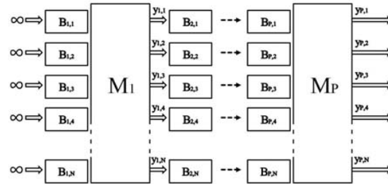
Fig. 3. Schematic of a flexible production line
