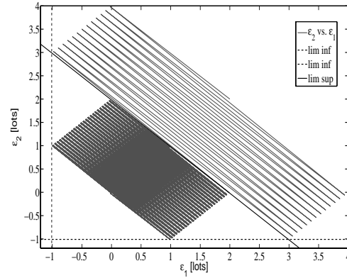
Fig. 2. Tracking Errors \varepsilon_2(k) vs. \varepsilon_1(k) , with v_{dj} = 0.99 [lots/time unit] and \mu_j = 2 [lot/ time unit].
