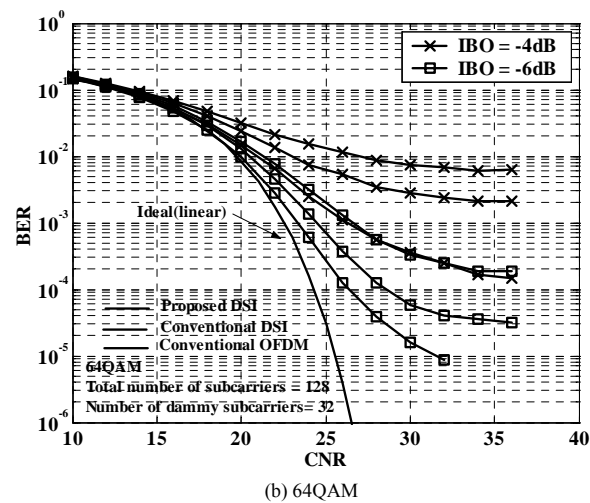
Fig. 9 BER performance of proposed DSI method in non-linear channel
